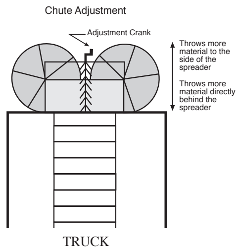
Figure 2. Adjustments for a spreader truck with spinner.
