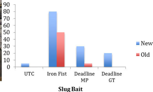
Figure 3. Bioassay 2 - Plastic bags containing potting soil, fresh dandelion leaves, 1 g of either fresh or 2-week old slug baits, and five slugs per bag. Bar graph to the right depicts % mortality of slugs after 72 hours exposure.
