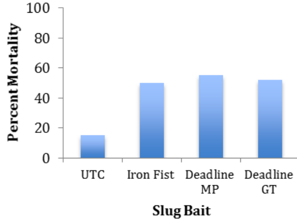
Figure 2. Potted corn bioassay to determine the efficacy of baits exposed to field conditions for 1 week. Bar graph to the right depicts percent mortality of slugs after 48 hours exposure.
