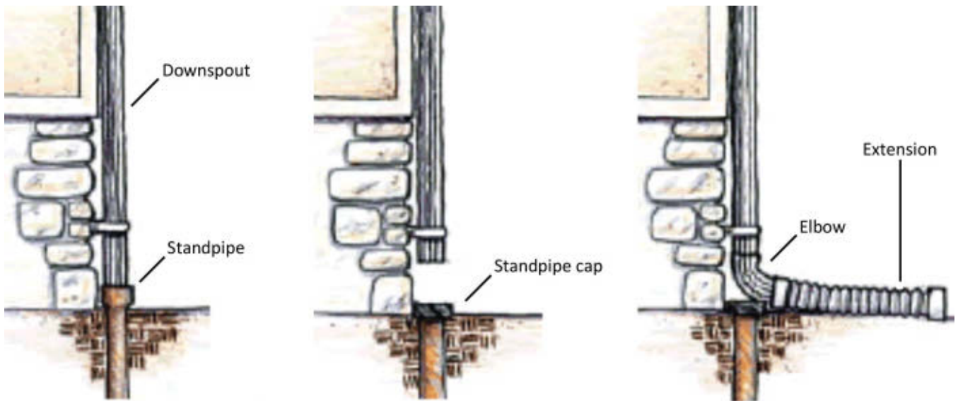
Downspout connected to standpipe.
